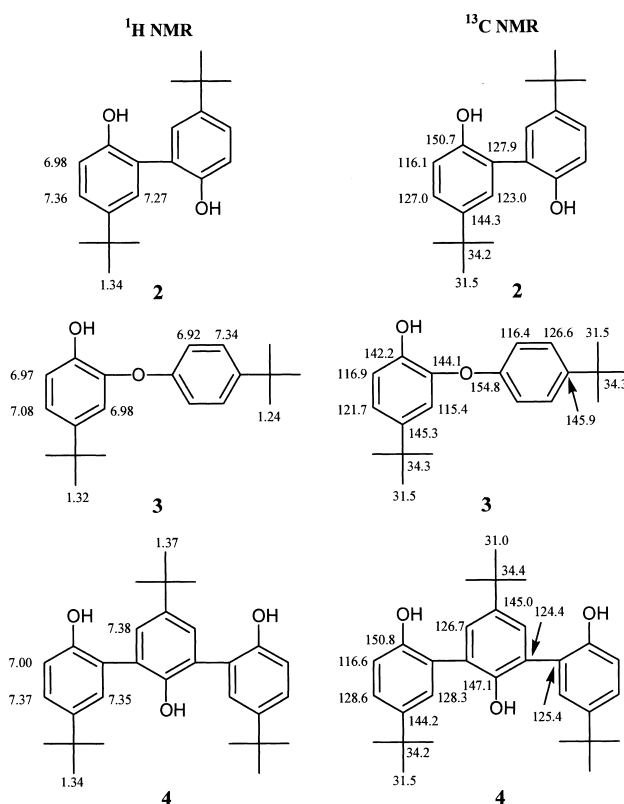
Fig. 2. Structure of isolated dimers ( 2 and 3 ) and trimer ( 4 ) and their assignment of ^1\text{H} and ^{13}\text{C} NMR peaks.
