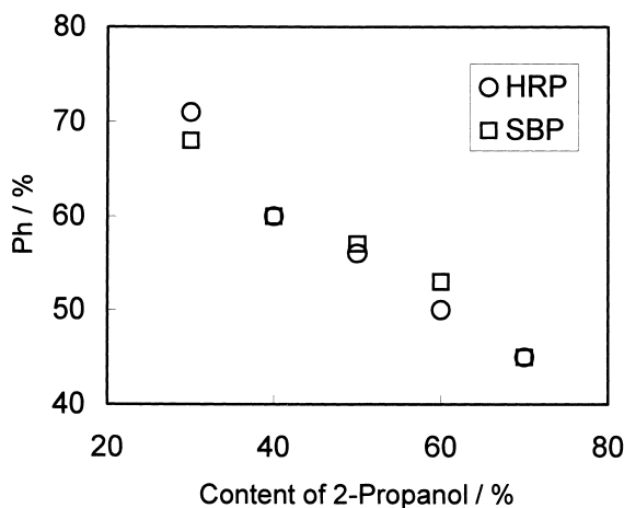
Fig. 5. Relationships between 2-propanol content and polymer structure in the peroxidase-catalyzed polymerization of 1 in a mixture of 2-propanol and phosphate buffer.
