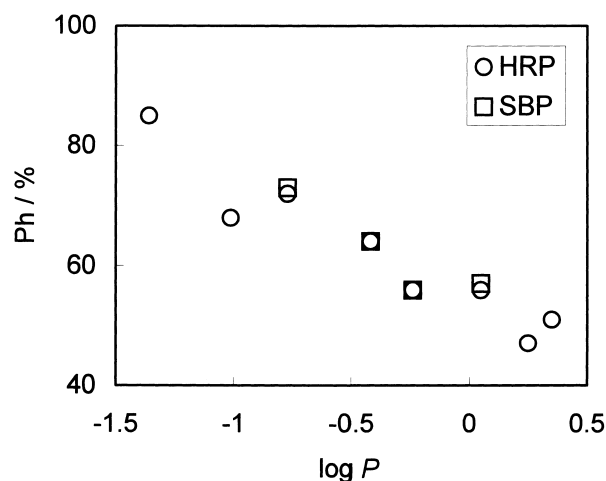
Fig. 6. Relationships between log P of organic solvents and polymer structure in the peroxidase-catalyzed polymerization of 1 in an equivolume mixture of organic solvent and phosphate buffer.
