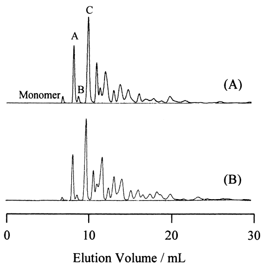
Fig. 1. HPLC traces of the product obtained from 1 in an equivolume mixture of methanol and phosphate buffer using (A) HRP and (B) SBP catalyst.
