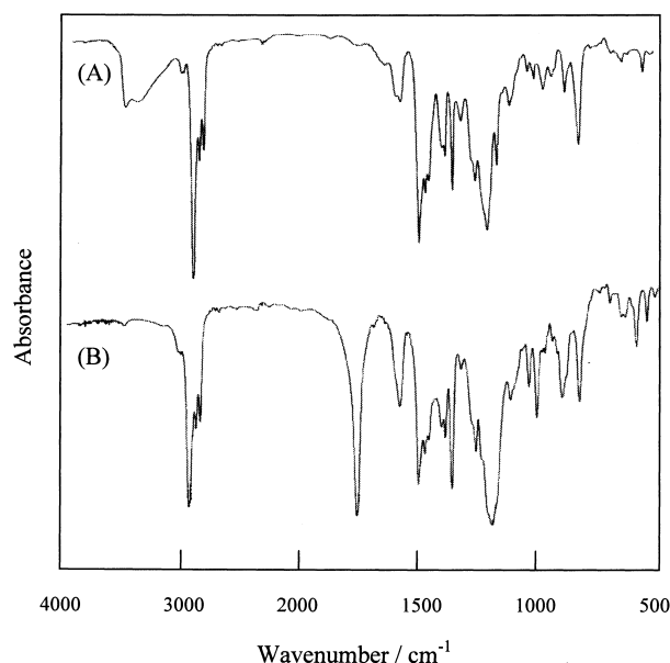
Fig. 4. FT-IR spectra of poly( 1 ) (entry 3 in Table 1) (A) before acetylation and (B) after acetylation.
