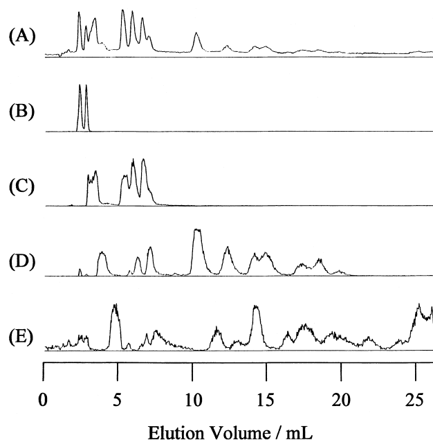
Fig. 3. LC/ESI-TOF mass chromatograms of poly( 1 ) with detector of (A) total ion, (B) m/z 321.1, (C) m/z 469.2, (D) m/z 617.3, and (E) m/z 765.4.
